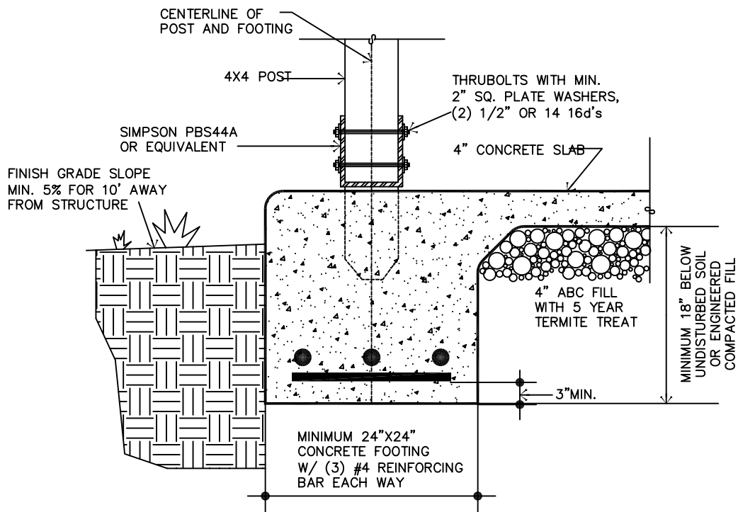
A - PATIO POST FOOTING
