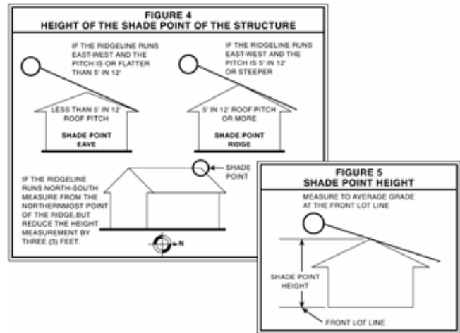
These figures from Clackamas County, Oregon, illustrate how solar access ordinances can provide detailed mechanisms for establishing and protecting access to sunlight for individual lots. (Image courtesy of Clackamas County, Oregon)
